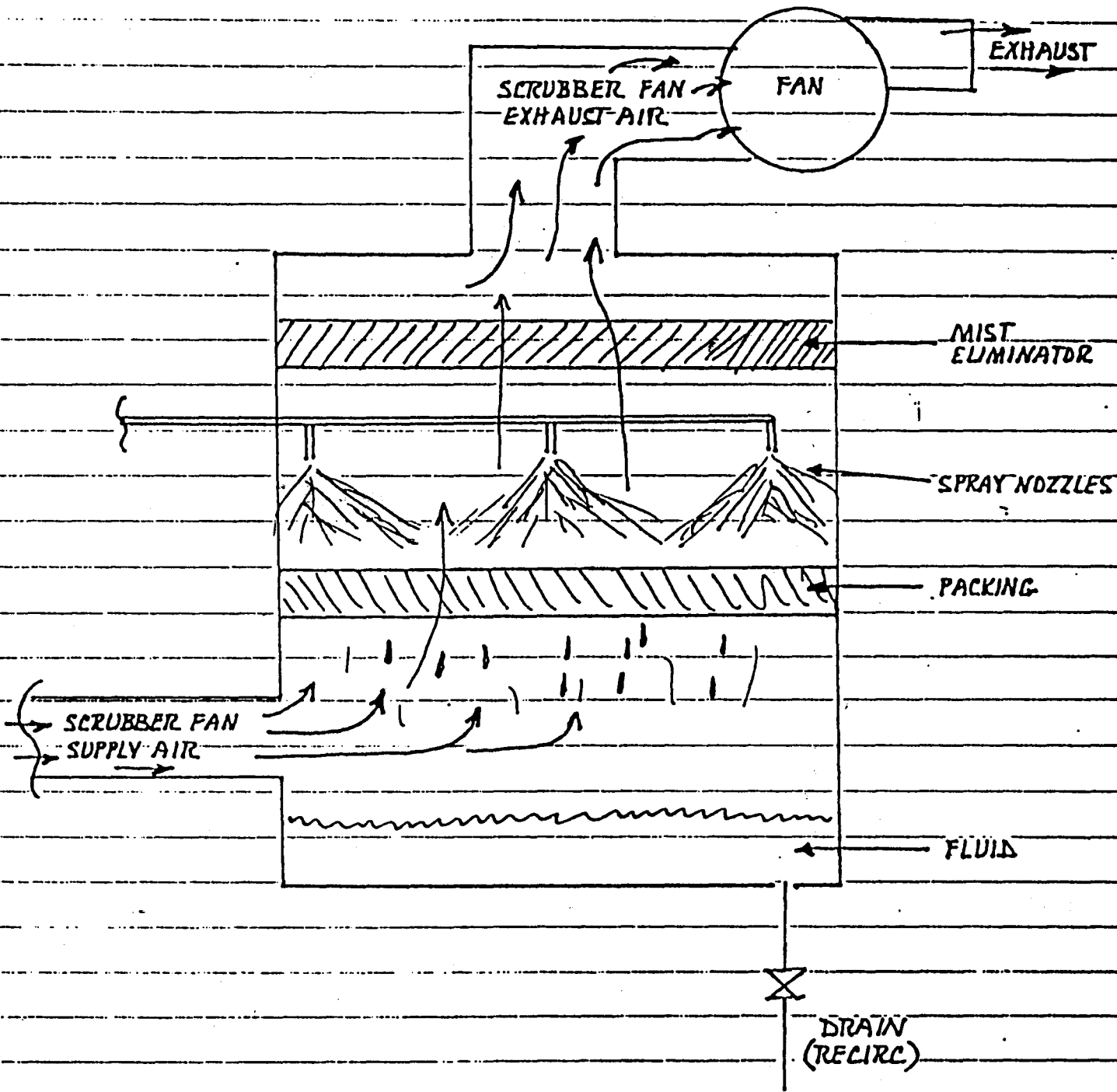
SIMPLIFIED SCRUBBER
